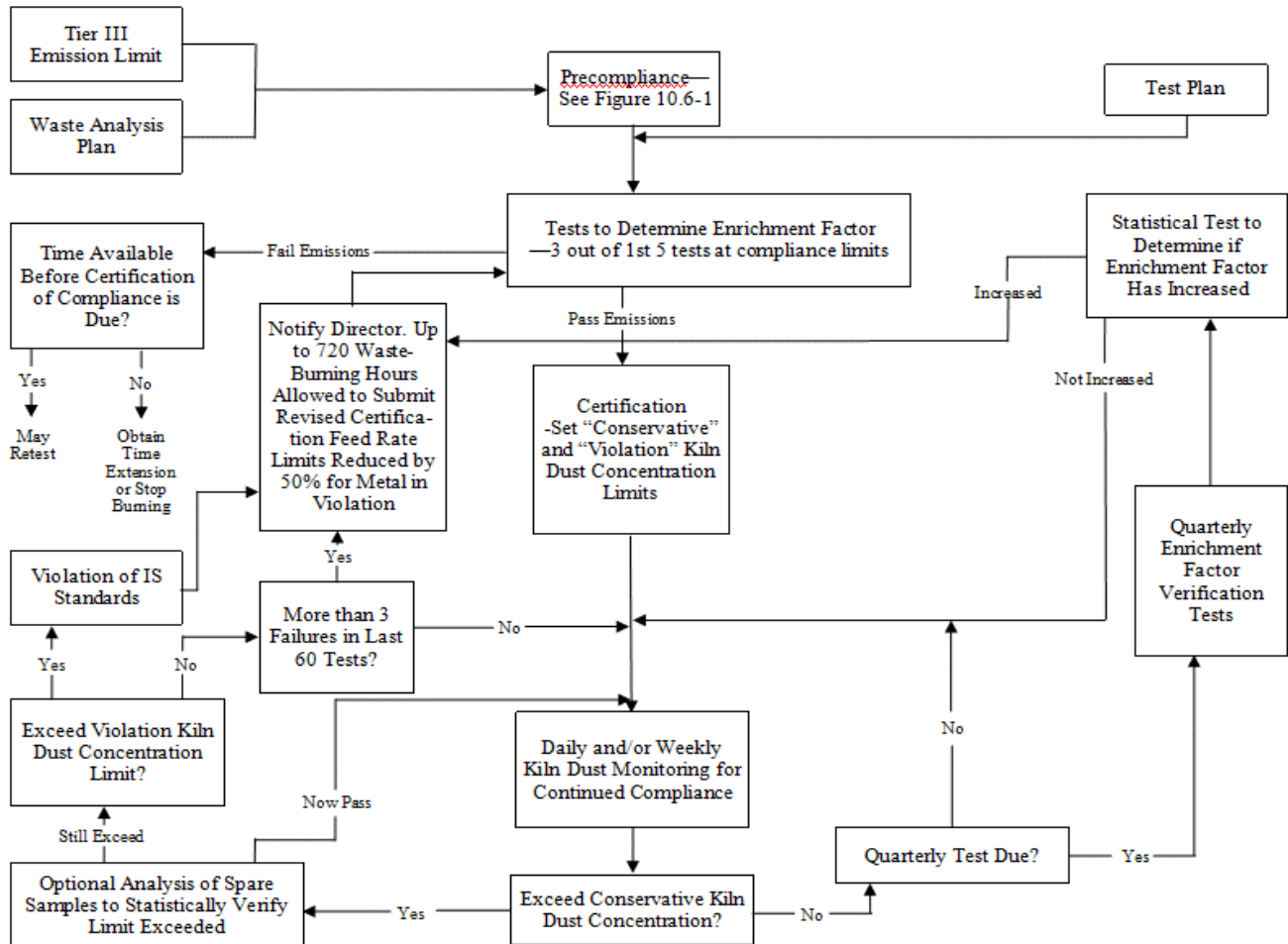
Figure 10.4-1 Compliance Implementation Flow Chart
