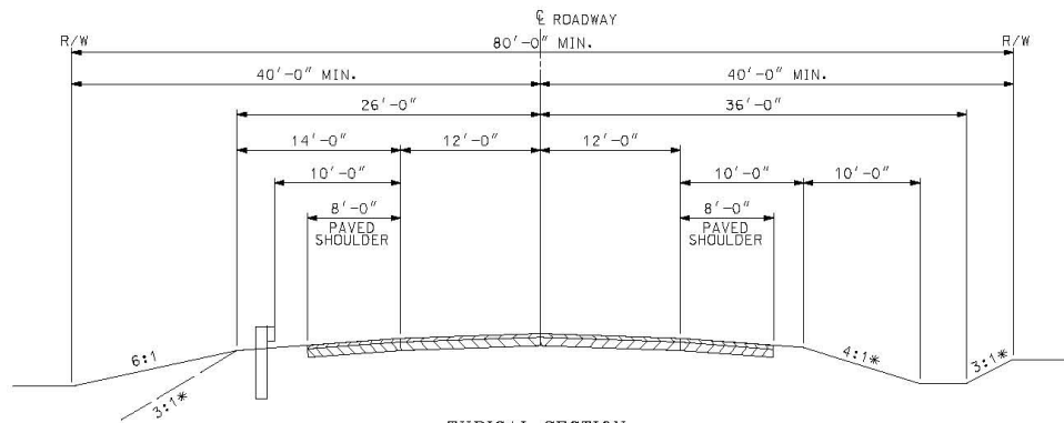
TYPICAL SECTION MINOR ARTERIAL TWO-LANE MAJOR OR MINOR COLLECTOR
