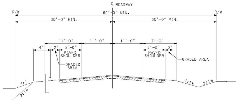
TYPICAL SECTION LOCAL ROAD
