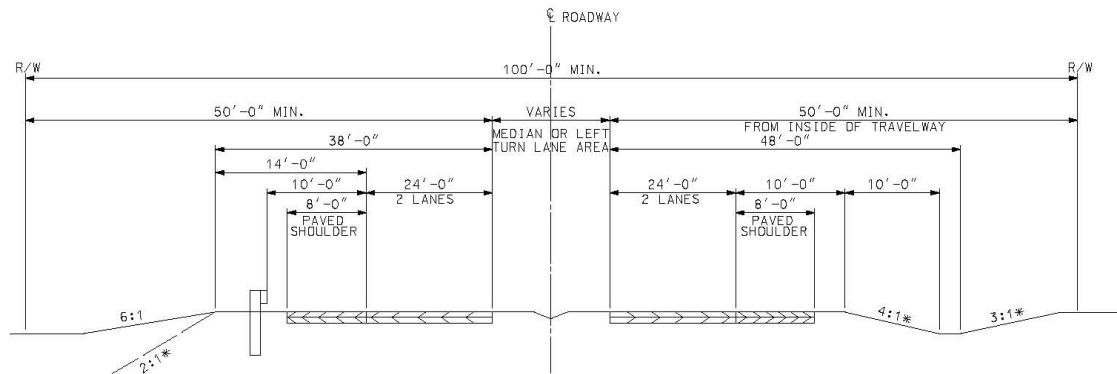
TYPICAL SECTION DIVIDED OR MULT-LANE UNDIVIDED FREEWAY OR EXPRESSWAY PRINCIPAL OR MINOR ARTERIAL
